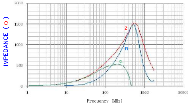
Z, R, XL vs. FREQUENCY
