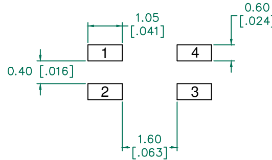
LAND PATTERNS FOR REFLOW SOLDERING
