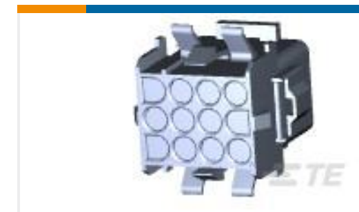
TE Part #770029-1 12P UMNLI IN-LINE CAP HSG KIT
