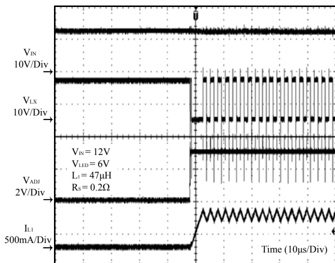
Figure 20 PWM On
