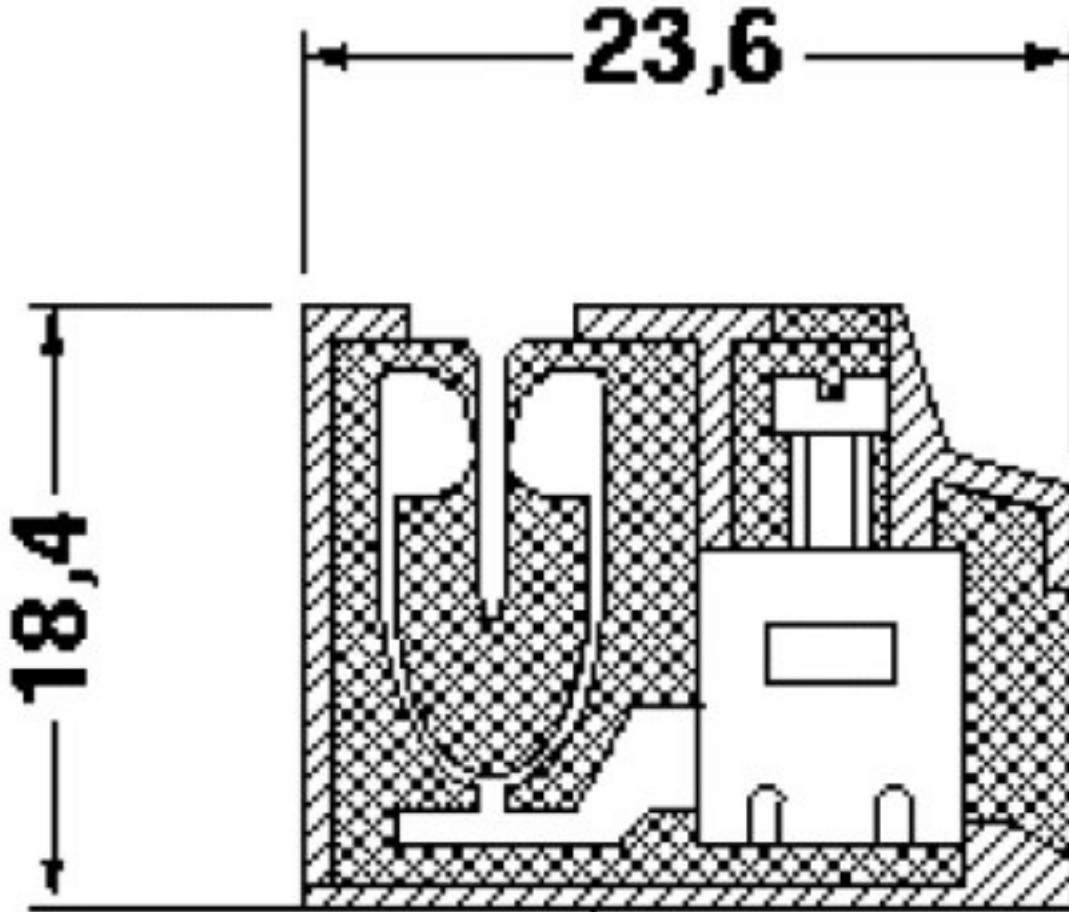
Dimensioned drawing
