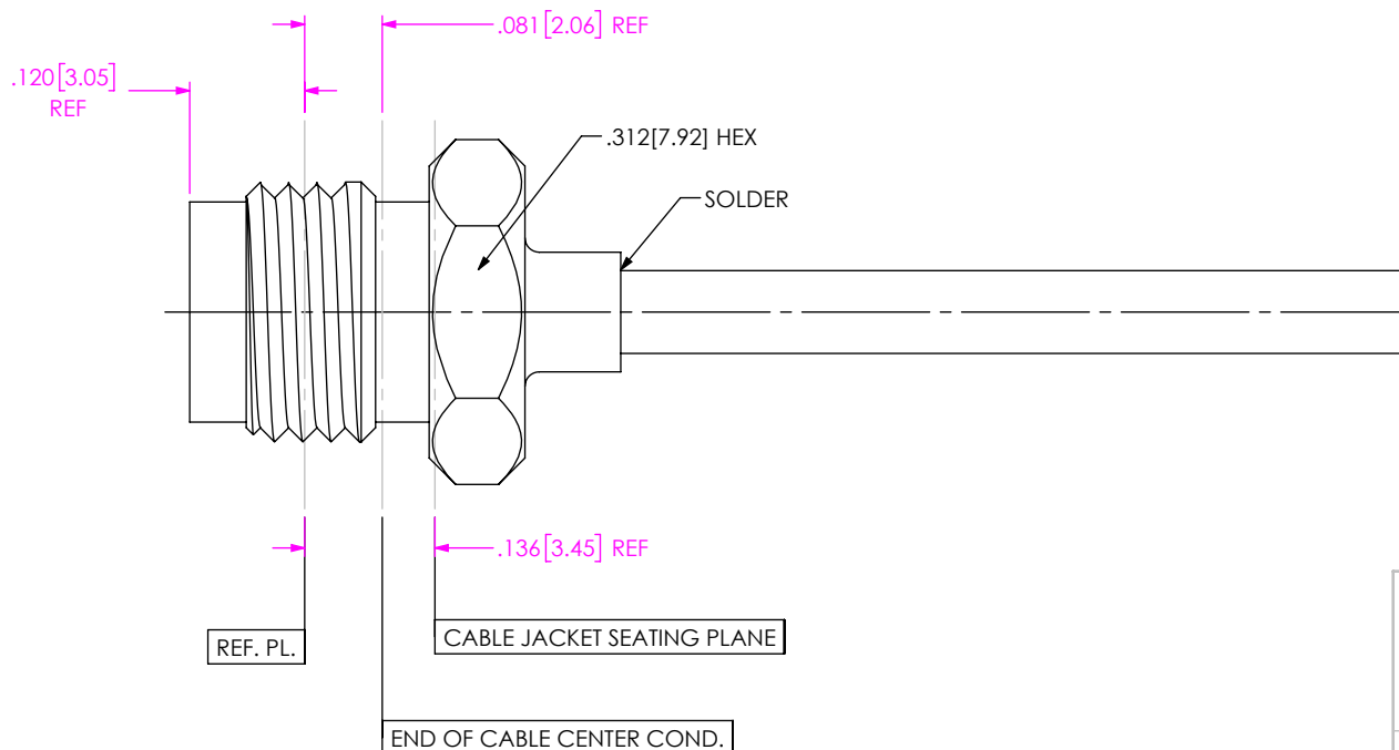
IN-PROCESS VIEW 3
