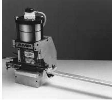
Tube-Fed Ribbon Cable Machine No. 856002-1
