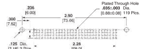
Recommended PC Board Layout for 1375965-5
