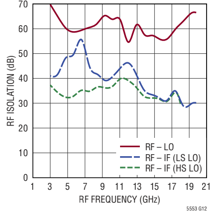
RF Isolation
