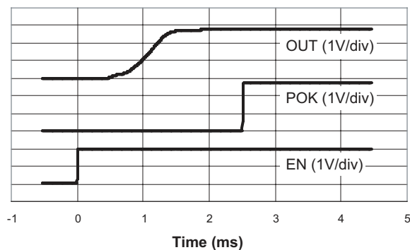
Turn-On With 10mA Load
