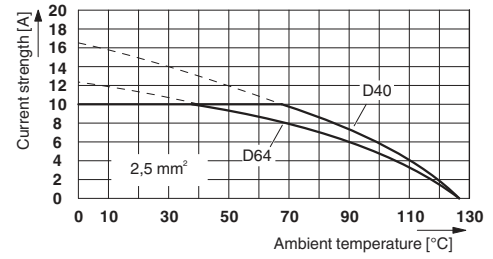
Derating diagram for 2.5 mm²
