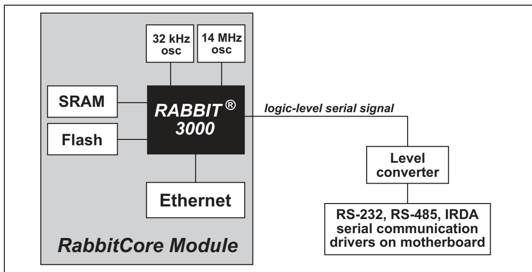
Figure 4. RCM3000 Subsystems
