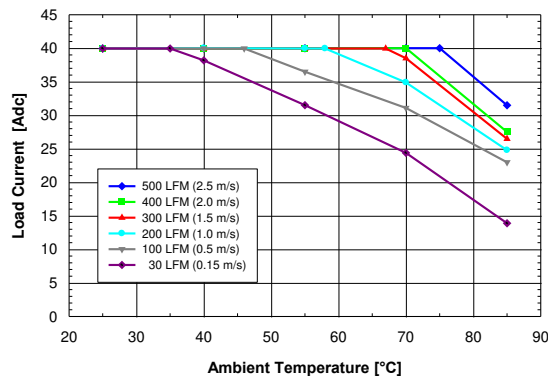
Figure 1. Available output current vs. ambient air temperature and airflow rates for converter DP8140G mounted horizontally with air flowing from input to output, V_{in} = 12\text{ V} , V_{out} = 3.3\text{ V} , and F_{sw} = 500\text{ KHz}
