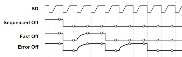
Figure 36. OK Severity Encoding Waveforms
