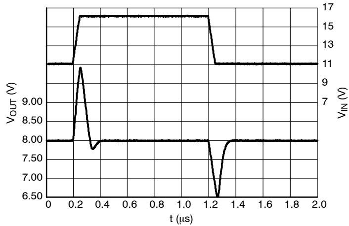
Figure 25. Line Transients, 8.0 V Version, t_R = t_F = 5 \mu s, I_{OUT} = 1 mA
