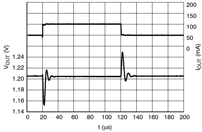
Figure 26. Load Transients, 3.0 V Version, I_{OUT} = 1 - 20 mA, t_R = t_F = 50 \mu s, V_{IN} = 6.0 V
