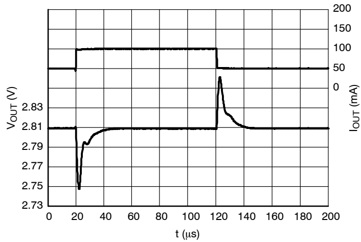
Figure 27. Load Transients, 5.0 V Version, I_{OUT} = 1 - 20 mA, t_R = t_F = 50 \mu s, V_{IN} = 8.0 V
