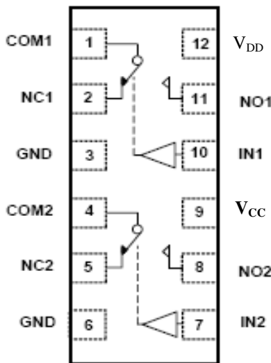
12-pin TDFN
