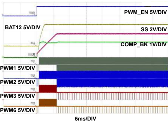
FIGURE 38. SOFT-START IN BUCK/DE/PD-ENABLED, 48V TO 12V, 6Ω LOAD ON BAT12
