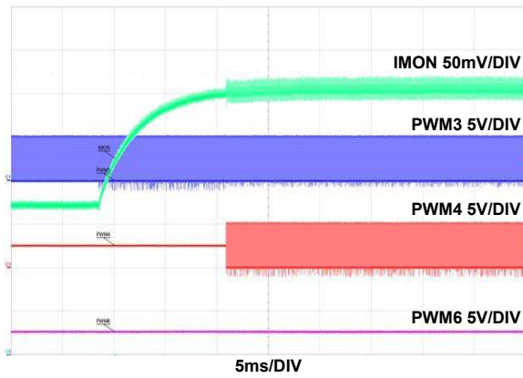
FIGURE 58. PHASE ADD TRANSITION IN BOOST/DE (3PH → 4PH), I_O = 4A \rightarrow 13A
