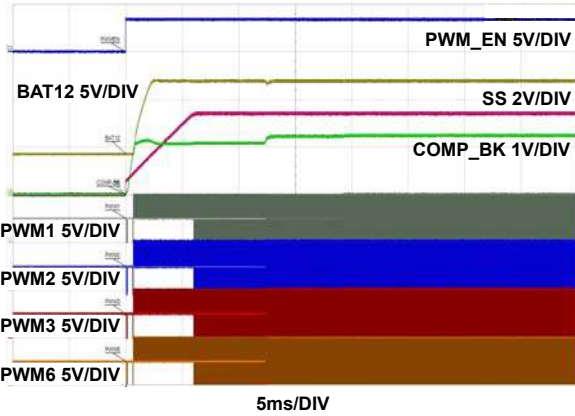
FIGURE 36. SOFT-START IN BUCK/FPWM/NO-PD, 48V TO 12V, 6Ω LOAD ON BAT12
