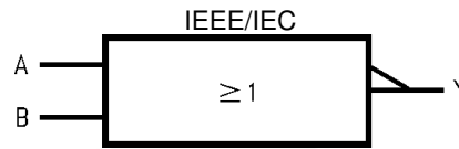
Figure 1. Logic Symbol
