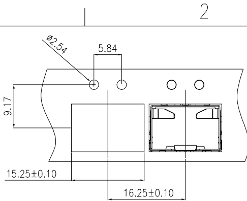
RECOMMENDED BEZEL CUT-OUT SINGLE SIDED APPLICATIONS
