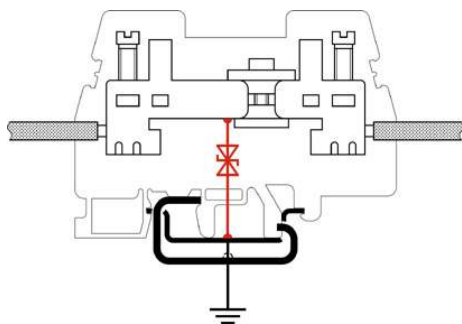
Schematic diagram
