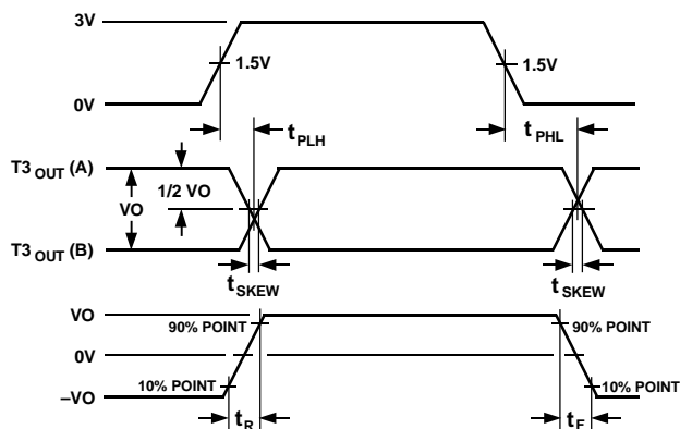
Figure 4. RS-422 Driver. Propagation Delay Rise/Fall Timing
