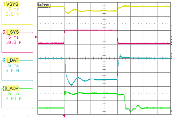
FIGURE 13. BOOST MODE, OUTPUT VOLTAGE LOOP TO ADAPTER CURRENT LOOP TRANSITION. V_{ADP} = 5V , MAXSYSTEMVOLTAGE = 8.496V, V_{BAT} = 7V , SYSTEM LOAD 0.5A TO 10A STEP, ADAPTERCURRENTLIMIT = 3A, CHARGECURRENT = 0A
