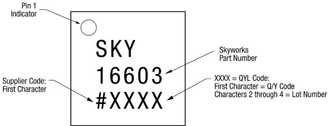
Figure 10. SKY16603-632LF Typical Part Markings
