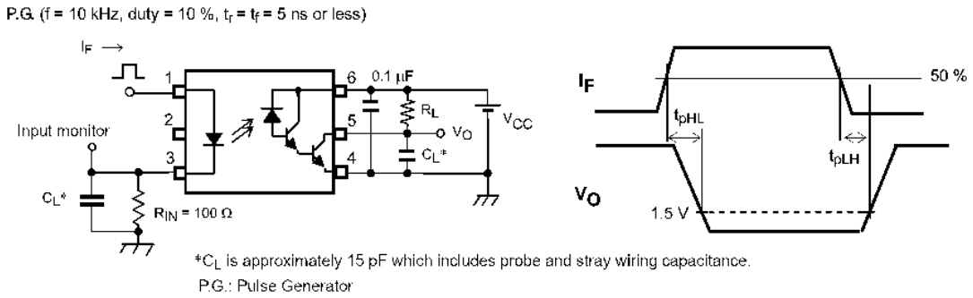
Fig. 12.1.1 Switching Time Test Circuit and Waveform
