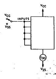
Fig. 13 - Quiescent device current test circuit.
