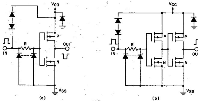
Fig. 1—a) Schematic diagram of CD4049UB, 1 of 6 identical units; b) Schematic diagram of CD4050B, 1 of 6 identical units.
