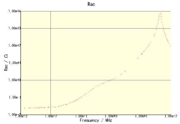
CLF6045T-6R8N-CA
