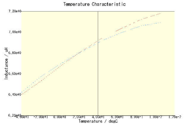
CLF6045T-6R8N-CA(DC = 0A)
