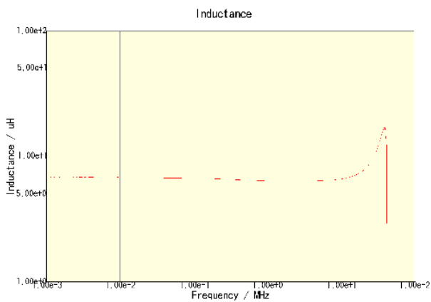
CLF6045T-6R8N-CA
