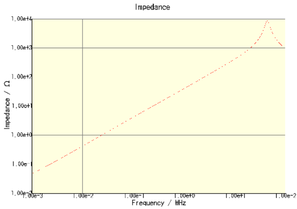
CLF6045T-6R8N-CA
