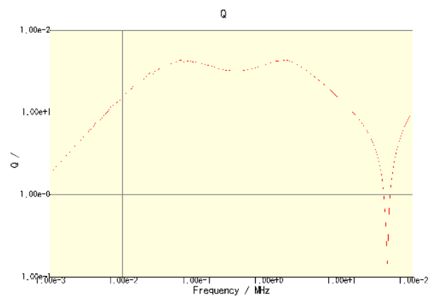
CLF6045T-6R8N-CA
