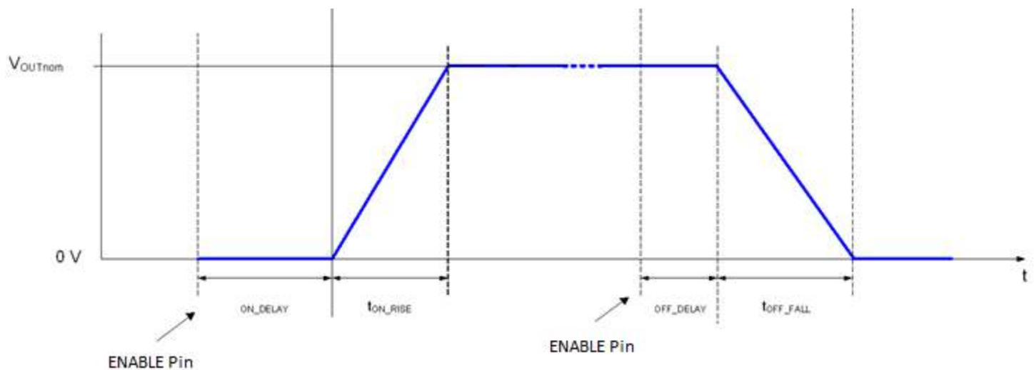
Figure 5: Power Sequencing
