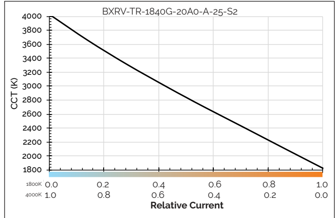
Figure 12: CCT vs. Relative Current
