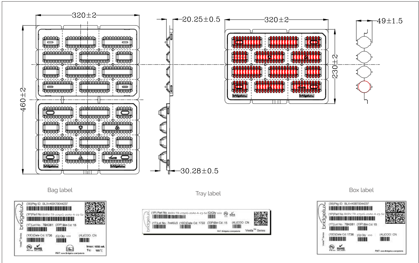
Figure 31: Packaging Specifications
