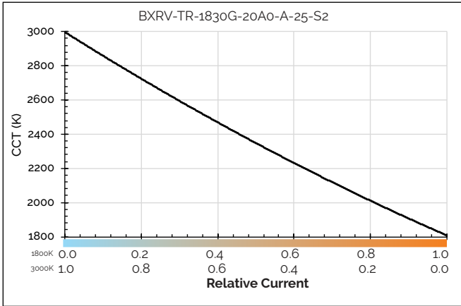
Figure 11: CCT vs. Relative Current
