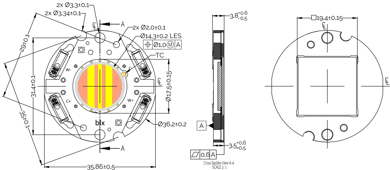
Figure 28: Mechanical Drawing Specifications
