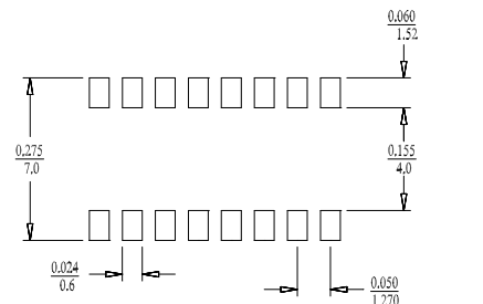
Mounting Pad
