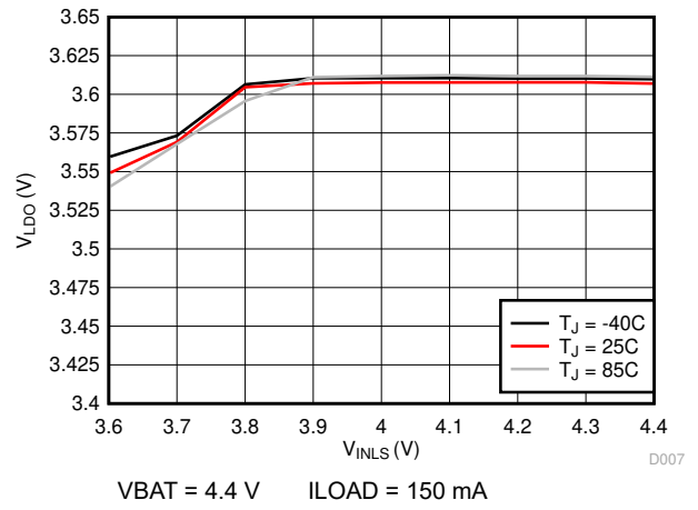
Figure 8-12. LDO Line Regulation (VLDO = 3.6 V)
