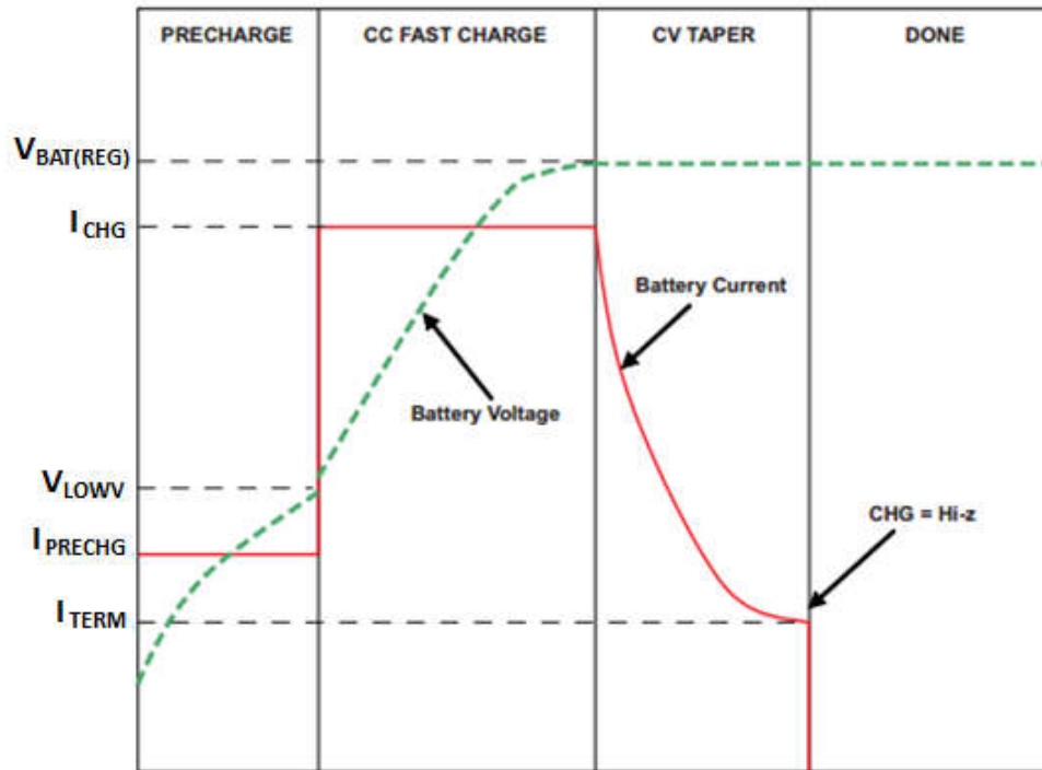
Figure 9-2. BQ25157 Typical Charge Cycle
