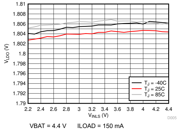
Figure 8-10. LDO Line Regulation (VLDO = 1.8 V)
