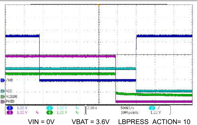
Figure 10-7. Ship Mode Entry with MR Bar Long Button Press
