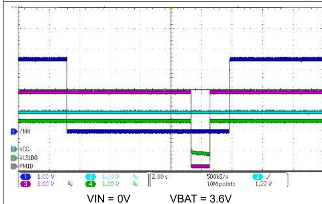
Figure 10-6. HW Reset on MR Bar Long Button Press
