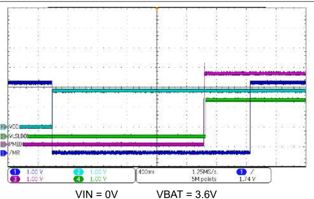
Figure 10-5. Power Up from Ship Mode with MR Bar Press
