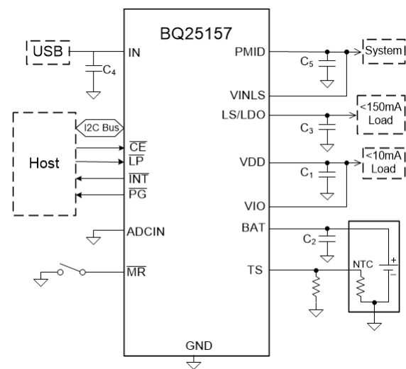
Simplified Schematic
