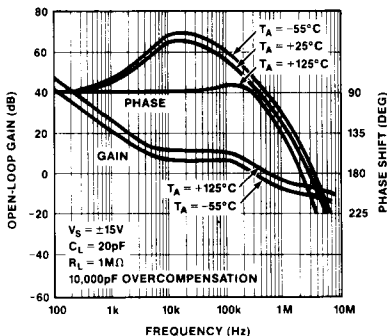
OPEN-LOOP GAIN, PHASE vs FREQUENCY ( C_{OC} = 10,000pF )
