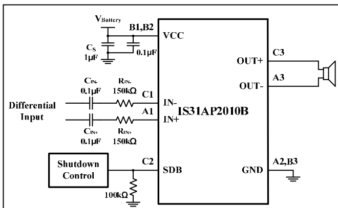
Figure 10 Differential Input
