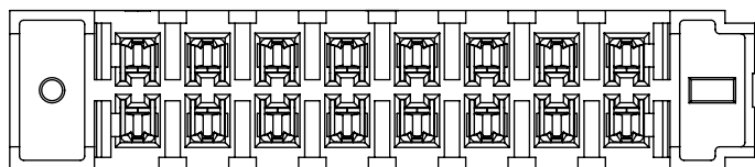
FIG 3 -GP: GUIDE POSTS IPBS-108-X1-X-D-GP SHOWN (DIFFERENT AS SHOWN, OTHERWISE SAME AS FIG 1)
