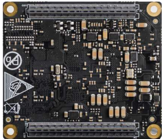
MYC-CZU3EG/4EV/5EV-V2 Bottom-view
