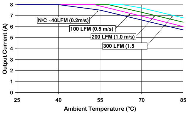
Figure 3. Output Current Derating vs Ambient Temperature & Airflow (Open Frame module) Vin = 24 V (airflow from pin 1 to pin 2)
