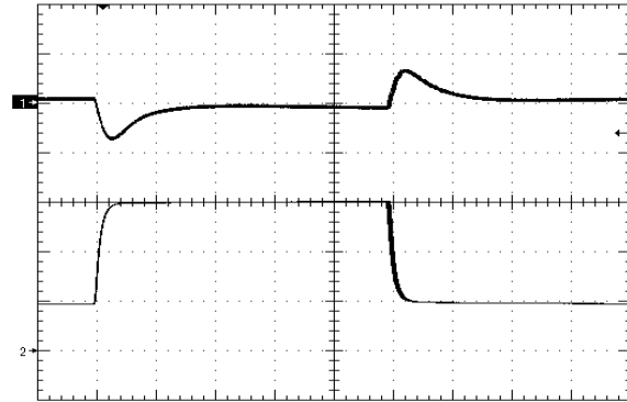
Figure 14. Load Transient Response 50mV/div, di/dt=0.2A/uS, 25% - 75% - 25% of full load +1000uF low ESR Oscon, time scale: 200uS/div. Ch1=Vout, Ch2=Iout (2A/div)
