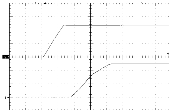
Figure 10. Startup Waveform via Line Voltage, time scale 4mS/div. Vin=Vin_nom, Iout=full load Cout=0uF, Ch1=Vout (2V/div), Ch2=Vin (20V/div)
