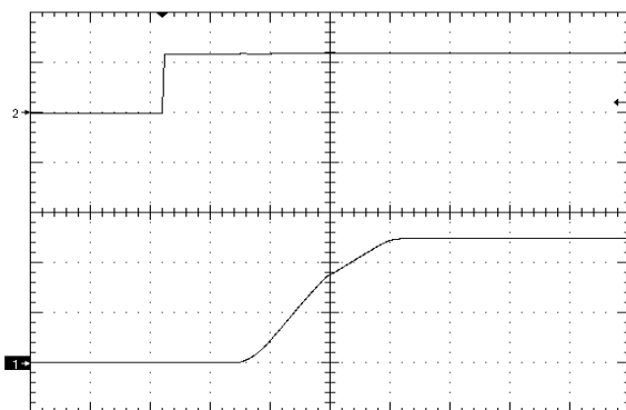
Figure 11. Startup Waveform via Enable Pin, time scale 4mS/div. Vin=Vin_nom, Iout=full load Cout=4700uF, Ch1=Vout (2V/div), Ch2=Enable (5V/div)
