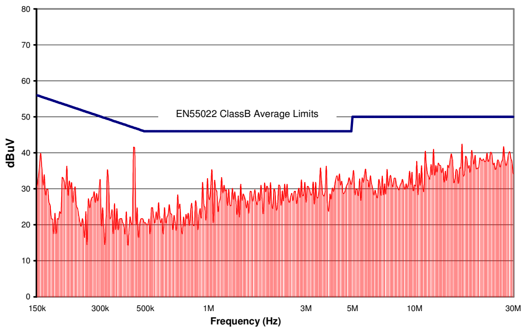
Figure 20. CP40_1180018 Conducted Emissions using above specified input filter. Vin = 24V, Full Resistive Load
