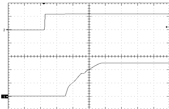
Figure 9. Startup Waveform via Enable Pin, time scale 4mS/div. Vin=Vin_nom, Iout=no load Cout=0, Ch1=Vout (2V/div), Ch2=Enable (5V/div)
