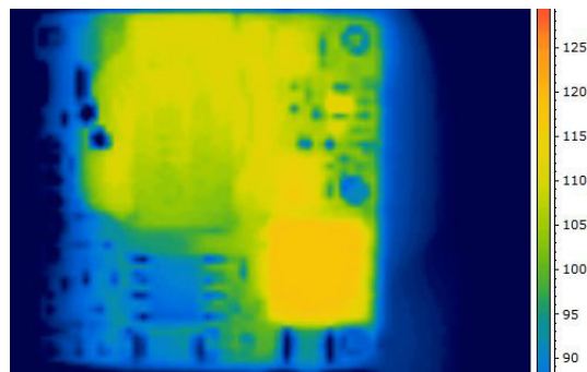
Figure 6. Thermal Image of CP40B1180018 8A output, 55C Ambient, 200lfm airflow, Vin = 24V, T max = 121 °C
