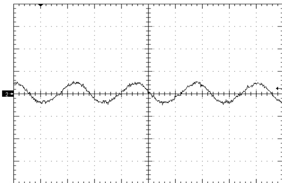
Figure 7. Input Reflected Ripple Current (20mA/div), time scale – 1uS/div. Vin=Vin_nom, full load (see Fig 15)
