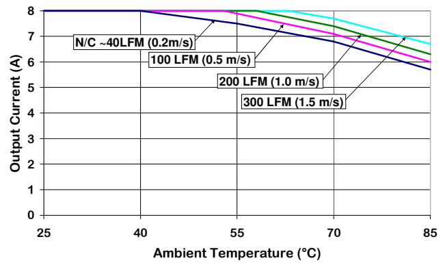
Figure 4. Output Current Derating vs Ambient Temperature & Airflow (Open Frame module) Vin = 12 V (airflow from pin 1 to pin 2)
