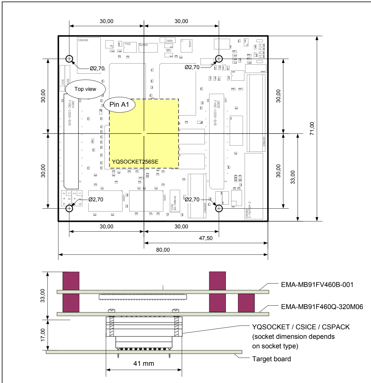
Figure 4-1: Mechanical Dimensions
