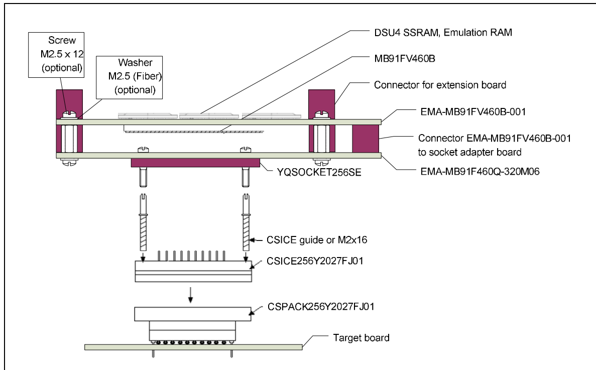
Figure 2-1: Installation
