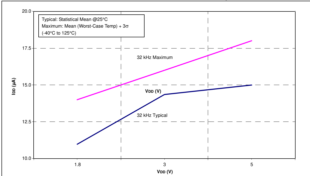
FIGURE 24-17: PIC16F722/3/4/6/7 I_{DD} vs. V_{DD} , LP MODE, V_{CAP} = 0.1 \mu F
