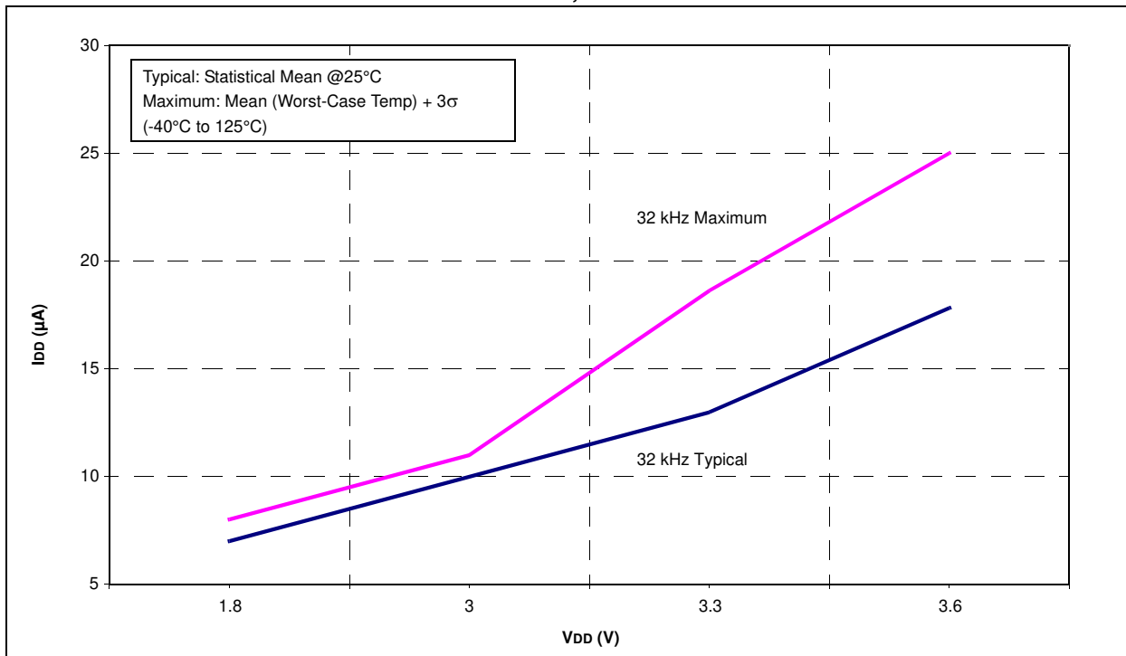
FIGURE 24-18: PIC16LF722/3/4/6/7 I_{DD} vs. V_{DD} , LP MODE
