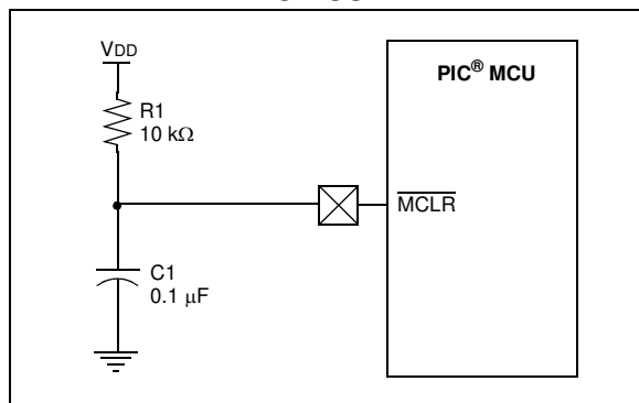
FIGURE 3-2: RECOMMENDED MCLR CIRCUIT
