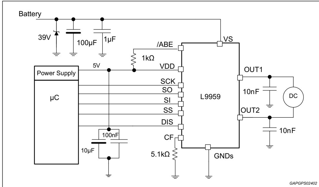
Figure 21. Application circuit
