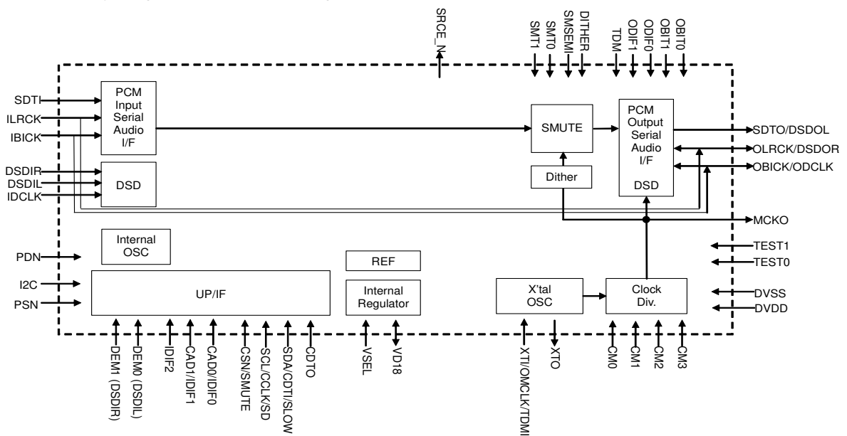
Figure 17. BYPASS Mode Master (PCMIN → PCMOUT)
