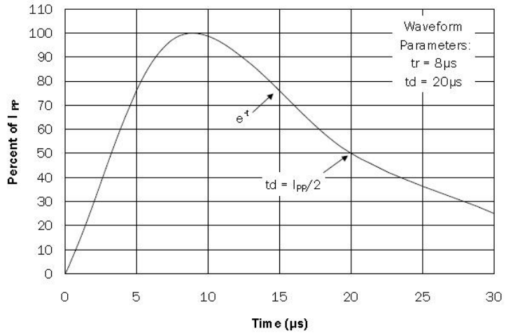
Fig.2 Pulse Waveform
