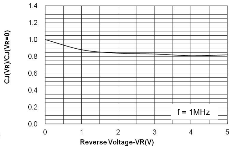
Fig. 4 Normalized Capacitance vs. Reverse Voltage
