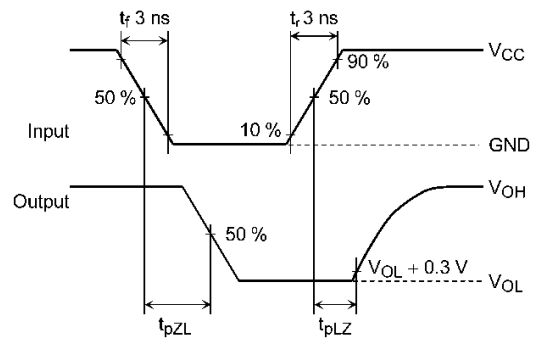
AC Waveform
