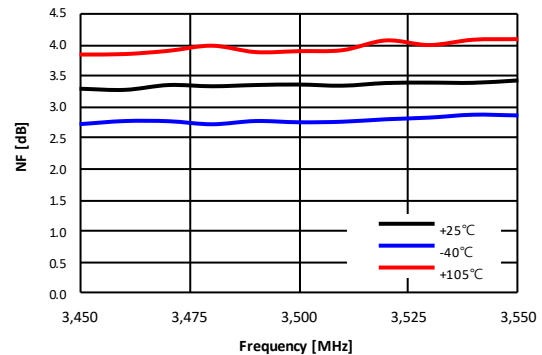
Figure 92. Noise Figure vs Frequency over Temperature
