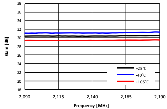
Figure 50. Gain vs. Frequency over Temperature
