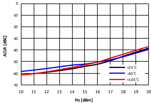
Figure 33. 3GPP LTE 20MHz ACLR vs Output Power over Temperature @900MHz
