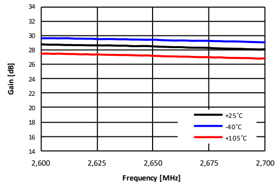
Figure 65. Gain vs. Frequency over Temperature
