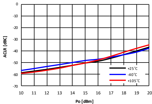
Figure 18. 3GPP LTE 20MHz ACLR vs Output Power over Temperature @700MHz
