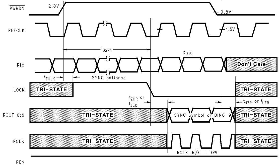
FIGURE 8. Deserializer PLL Lock Times and PWRDN TRI-STATE Delays
