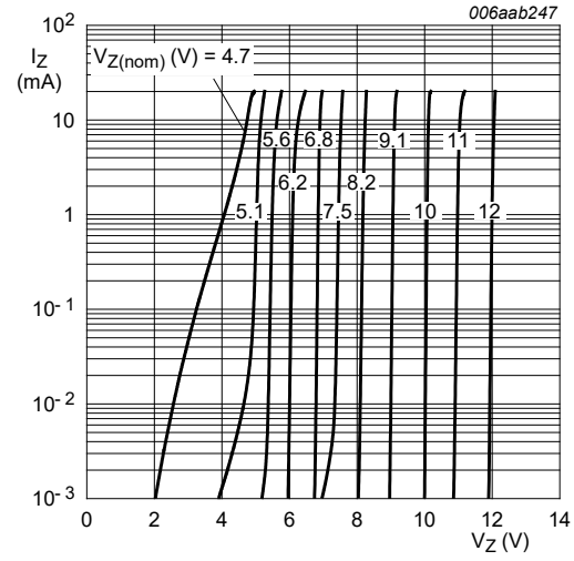
Fig. 6. Working current as a function of working voltage; typical values
