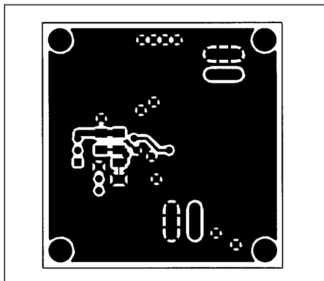
Figure 5. MAX1771 EV Kit PC Board Layout—Solder Side
