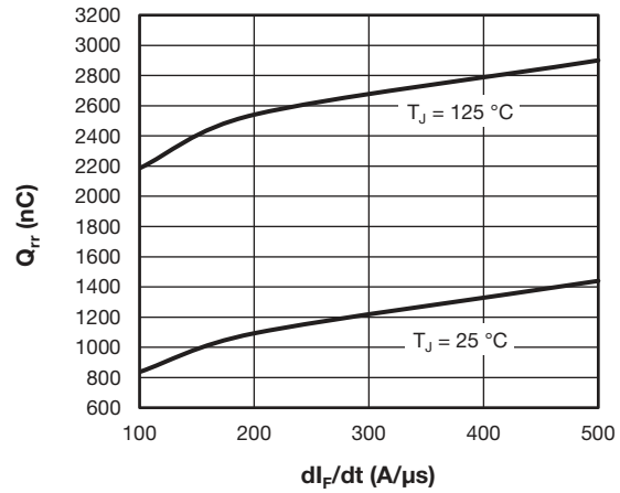
Fig. 16 - Typical Diode Reverse Recovery Charge vs. di/dt V_{rr} = 400\text{ V} , I_F = 50\text{ A}
