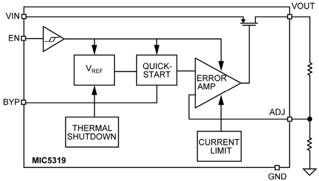
MIC5319 Block Diagram – Adjustable
