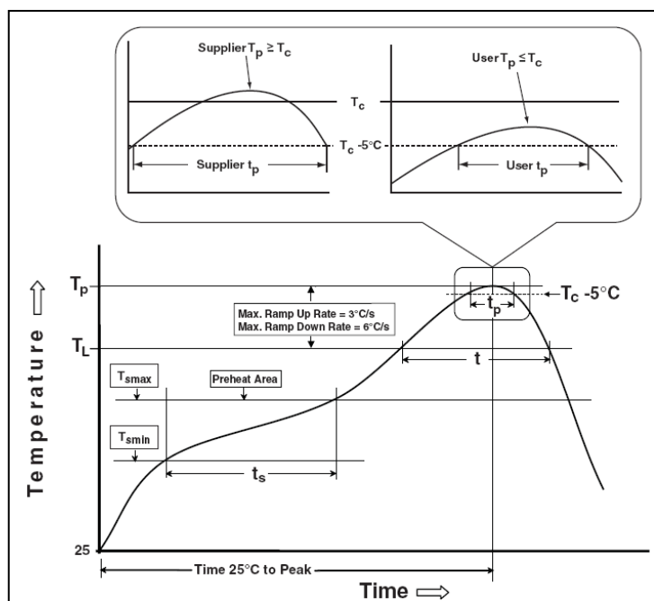
Figure 11 Classification Profile
