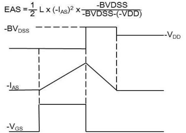
Fig.8 E_{AS} Waveform
