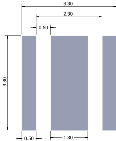
Recommended PCB Footprint
