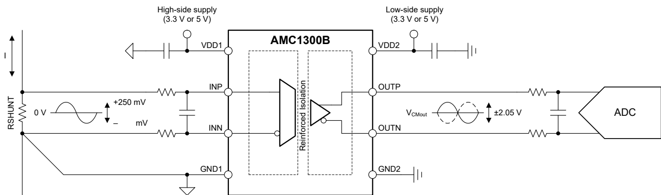
Simplified Schematic
