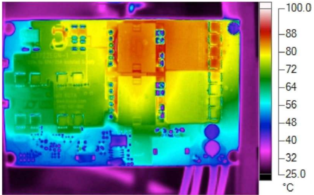
Figure 4. Thermal Map, 48V IN , 12V at 35A OUT , 200LFM, Frontside
