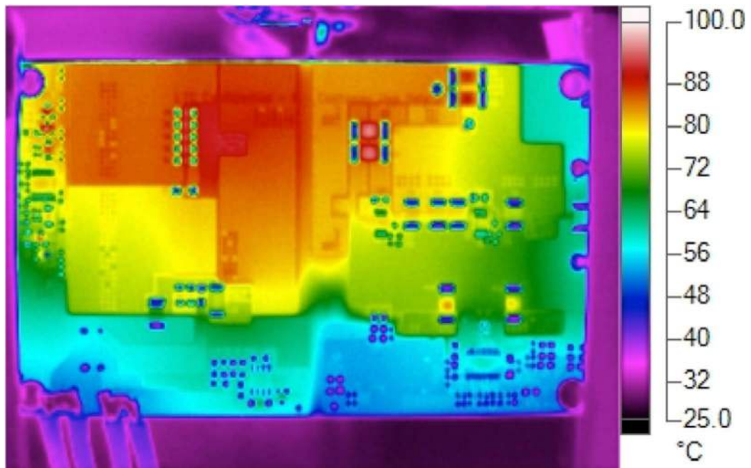
Figure 5. Thermal Map, 48V IN , 12V at 35A OUT , 200LFM, Backside
