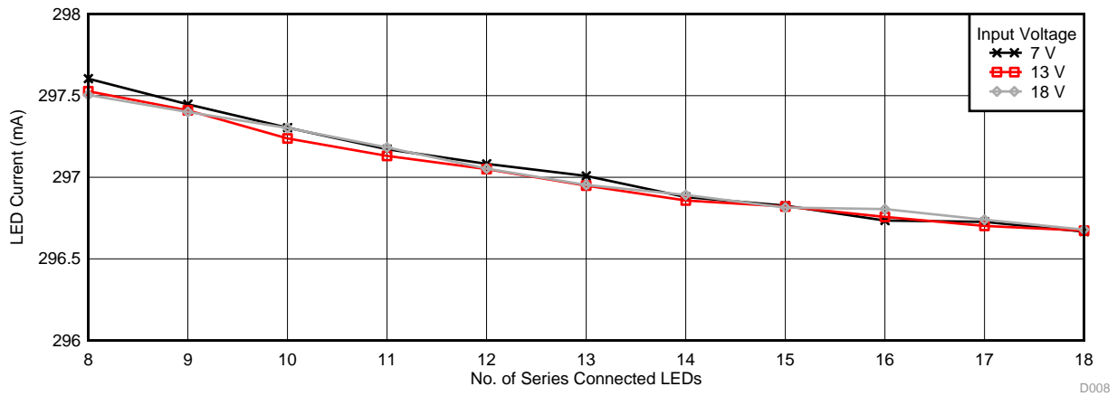
Figure 10. Output LED Current vs LED String Configuration ( V_{IADJ} = 1.26 \text{ V} )
