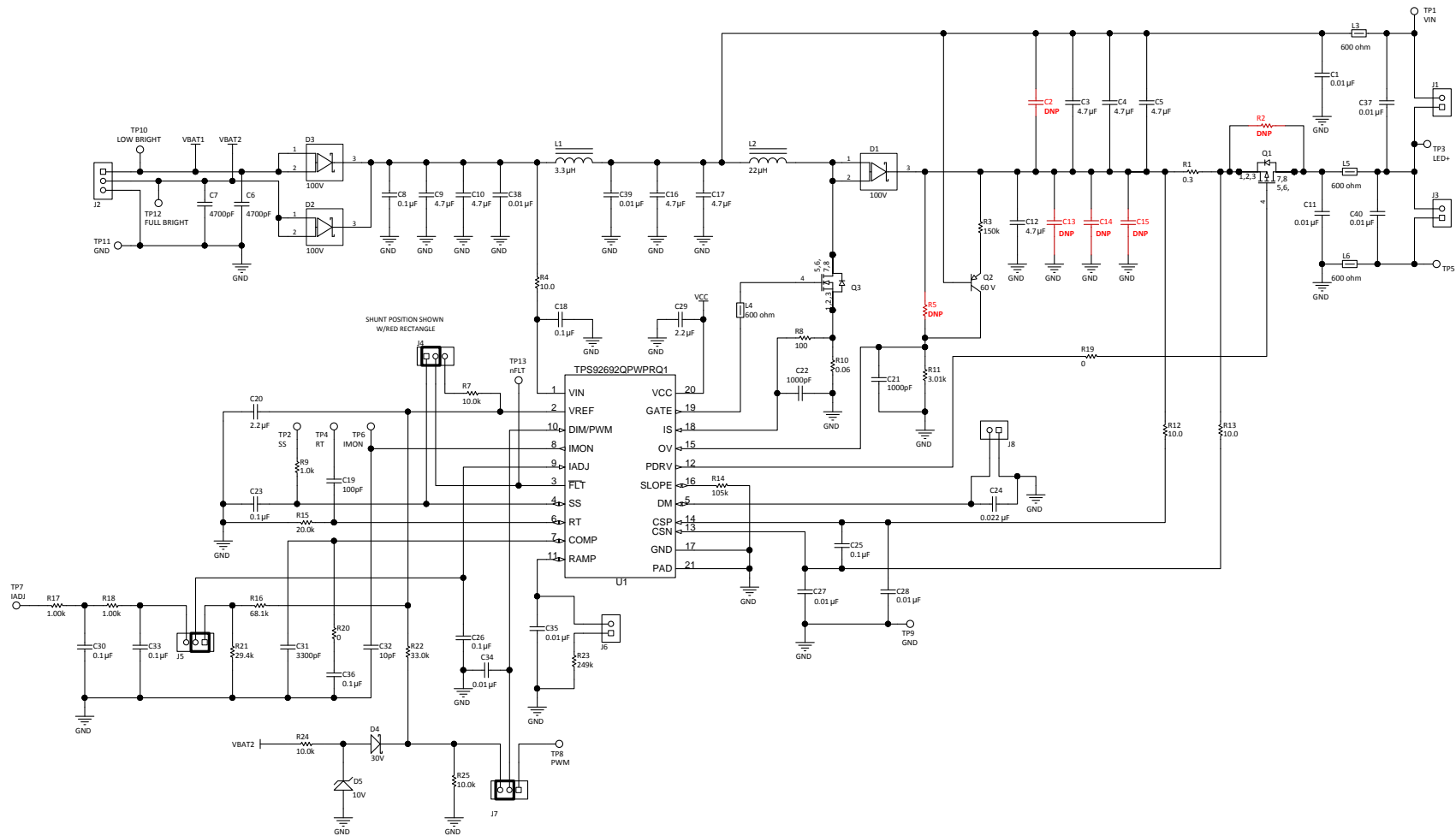
Figure 23. TPS92692EV-880 Schematic: Configured as a Buck-Boost LED Driver
