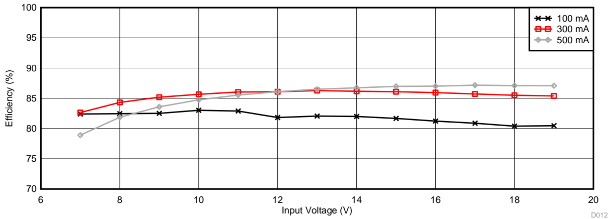
Figure 24. Efficiency vs Input Voltage (Number of Series-Connected LEDs = 7)
