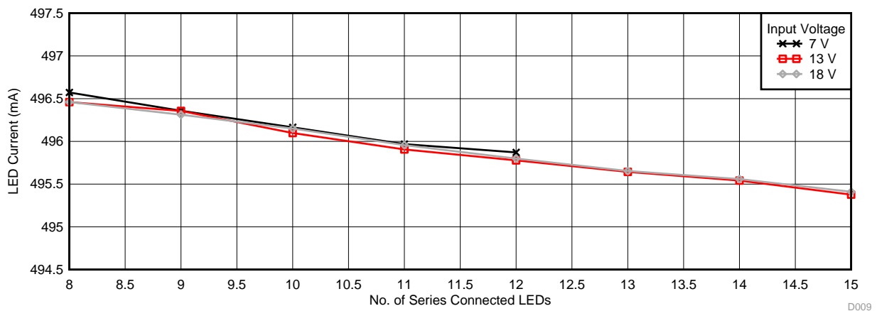
Figure 11. Output LED Current vs LED String Configuration ( V_{IADJ} = 2.1 \text{ V} )
