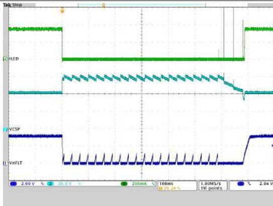
Ch1: FLT output Ch2: GSP pin voltage Ch4: LED current; Time: 100 ms/div Figure 20. LED Open-Circuit Fault
