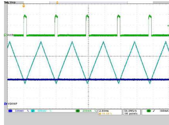
Ch1: Dim/PWM voltage Ch2: RAMP pin voltage Ch4: LED current; Time: 2 ms/div Figure 17. Analog-to-PWM Dimming Transient
