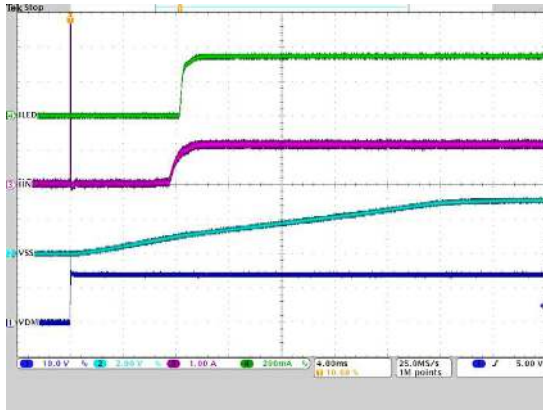
Ch1: Input voltage; Ch2: Soft-start (SS) voltage Ch3: Input current Ch4: LED current; Time: 4 ms/div Figure 16. Startup Transient
