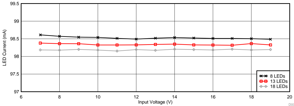
Figure 6. Output LED Current vs Input Voltage ( V_{IADJ} = 420 \text{ mV} )
