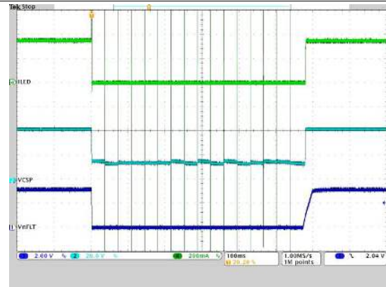
Ch1: FLT output Ch2: GSP pin voltage Ch4: LED current; Time: 100 ms/div Figure 21. LED Short-Circuit Fault
