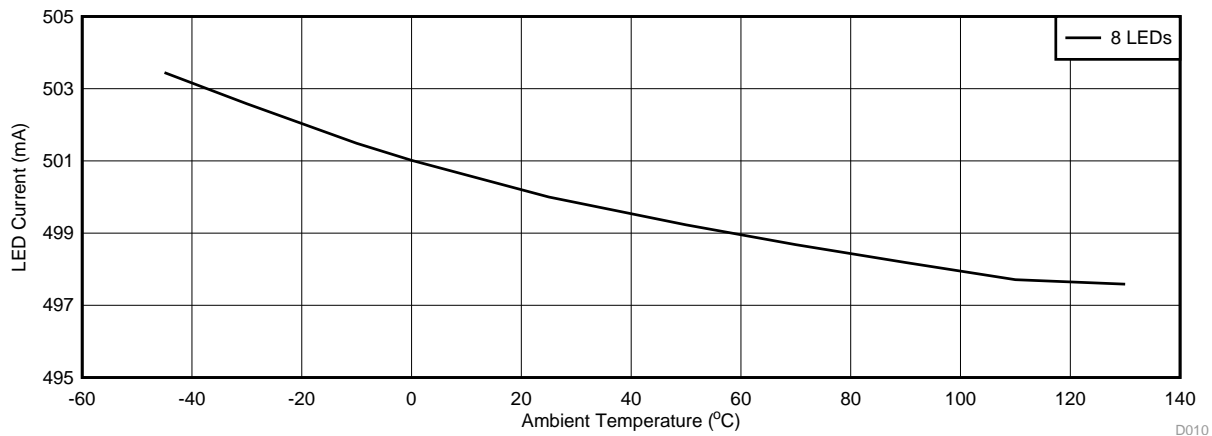
Figure 12. LED Current vs Ambient Temperature ( V_{IN} = 13\text{ V} , Number of LEDs in Series = 8)
