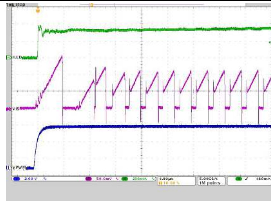
Ch1: External PWM input voltage Ch3: Switch sense current resistor voltage Ch4: LED current; Time: 4 µs/div Figure 19. PWM Dimming Transient (Zoomed)
