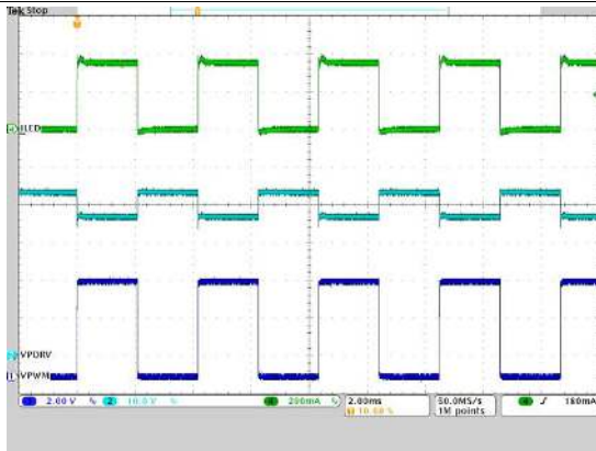
Ch1: External PWM input signal Ch2: PDRV voltage Ch4: LED current; Time: 2 ms/div Figure 18. Direct PWM Dimming Transient
