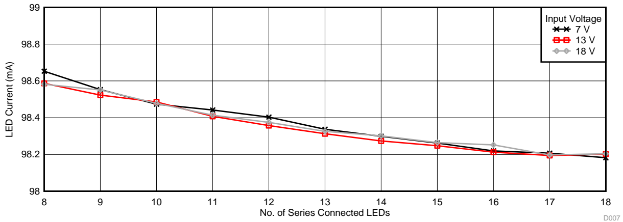
Figure 9. Output LED Current vs LED String Configuration ( V_{IADJ} = 420 \text{ mV} )
