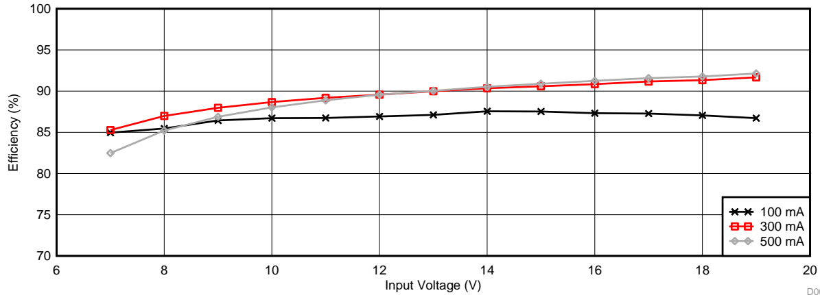
Figure 3. Efficiency vs Input Voltage (Number of Series-Connected LEDs = 8)
